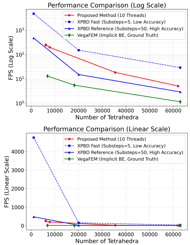
FIGURE 7. Overall performance trend across Frame rate versus mesh scales (log-scale FPS axis) for the proposed method (10 threads), XPBD under the Fast and Reference substep configurations defined in Section IV-A, and VegaFEM. The proposed method maintains better real-time performance than VegaFEM over a broad tetrahedral range and still retains basic interactivity on larger-scale models.
